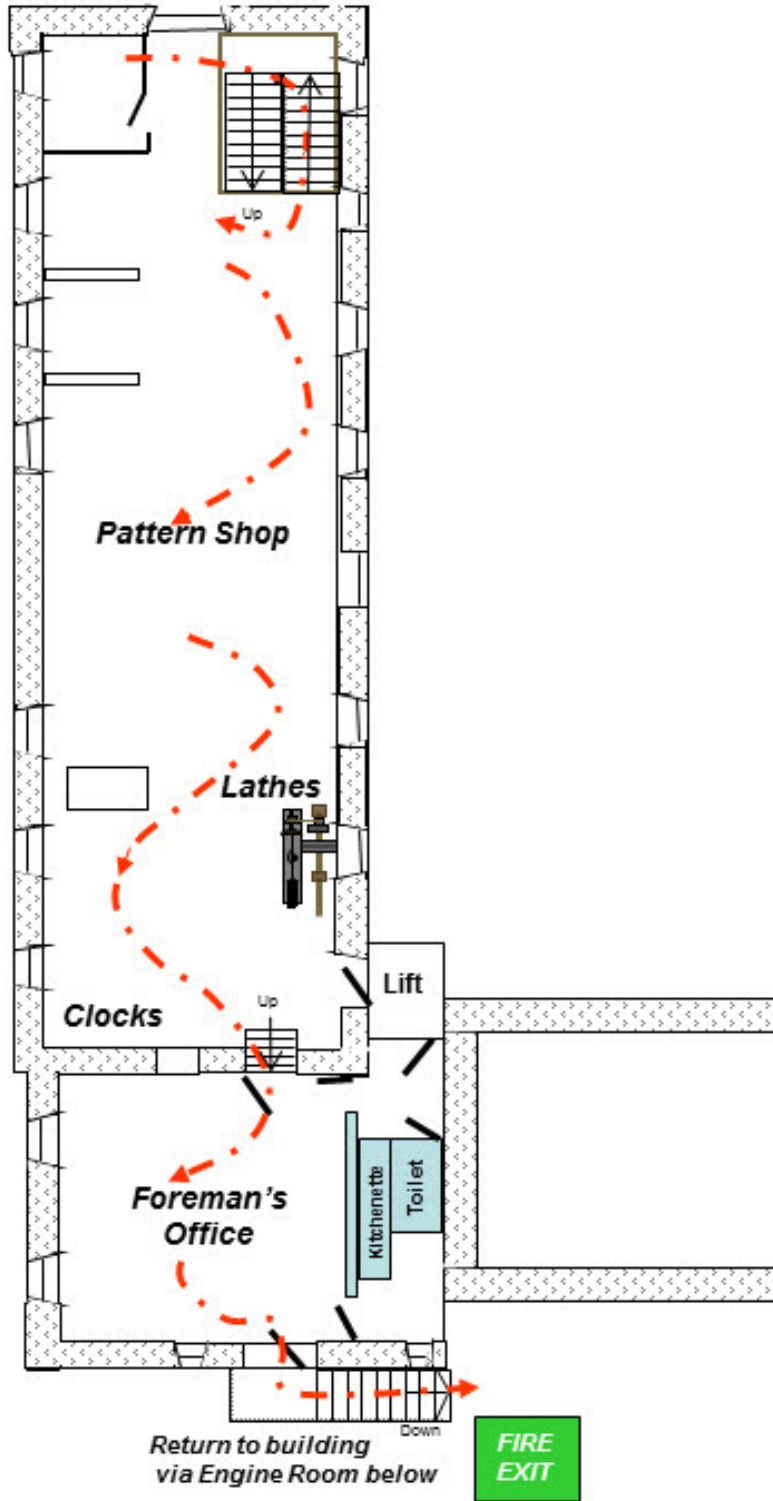
Figure 2 Combe Mill Upper Floor Plan
